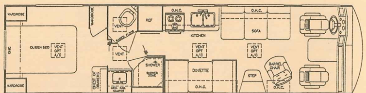
MODEL 8323 (Queen or Twin Bed Opt. Available)
